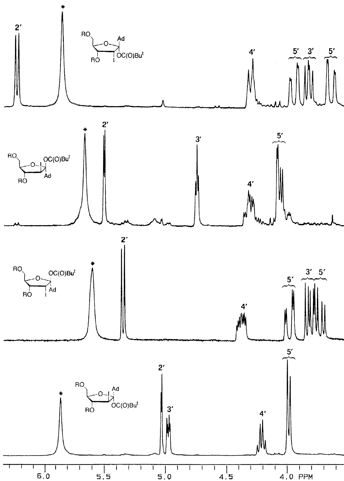
Figure 1. ^1\text{H} NMR spectra of the nucleosides ( \text{R} = \text{TBDMS} ) in the region of sugar resonances. (*) Resonance signal from \text{NH}_2 group of adenine.
